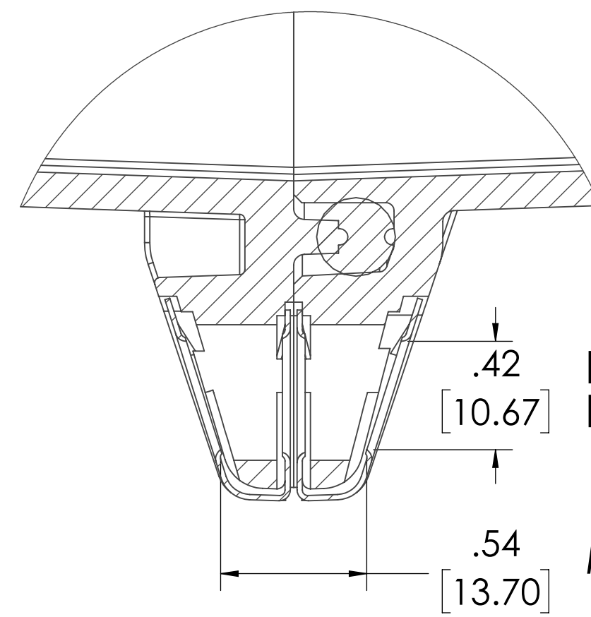
SECTION C-C SCALE 2 : 1
